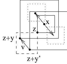
FIGURE 7. Sketch of the situation in Lemma 25.
