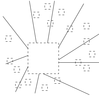
FIGURE 5. Regions in dimension 2.
