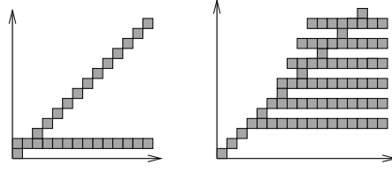
FIGURE 2. Examples of sets definable in Presburger arithmetic.
