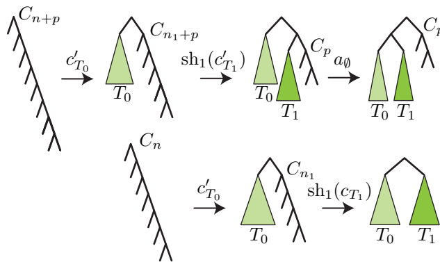
FIGURE 15. For T a size n tree, c_T describes how to construct T from the right-comb C_n , and c'_T describes how to construct T \wedge C_p from C_{n+p} ; the figure illustrates the recursive definition of c'_T (above) and c_T (below) for T = T_0 \wedge T_1 , with n_1 denoting the size of T_1 .
