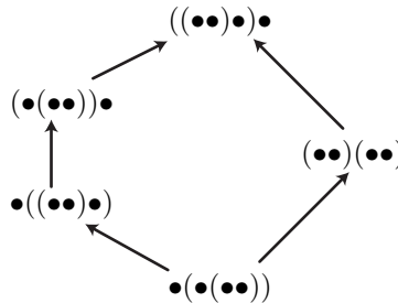
FIGURE 1. The Tamari lattice \mathcal{T}_3 made by the five ways of bracketing a four variable parenthesized expression.
