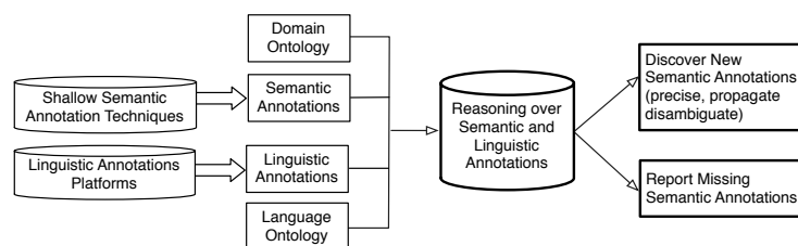
Fig. 1. Framework Overview: Reasoning Approach for Fine-grained Semantic Annotation of Text
