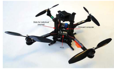
Fig. 2. The Pelican quadcopter
