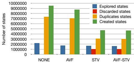
Figure 5: Impact of heuristics on the search.
