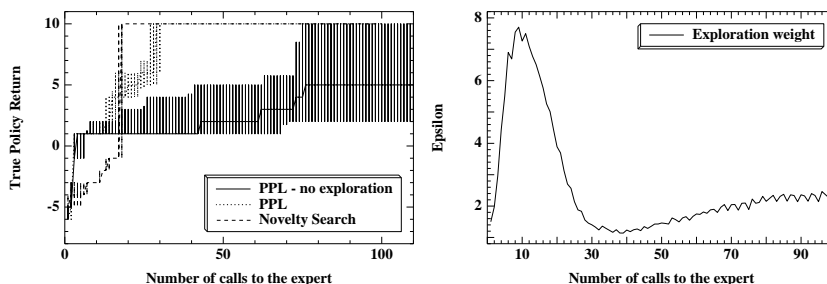
Fig. 2. 2D RiverSwim: Performance of PPL and Novelty-Search , averaged over 41 runs with std. dev (left); average weight of the exploration term \alpha_t in PPL (right).
