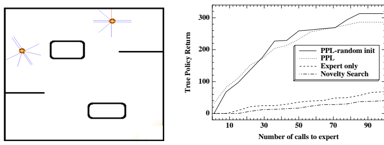
Fig. 5. Synchronous exploration: the arena (left) and the best average performance out of 41 runs (right).
