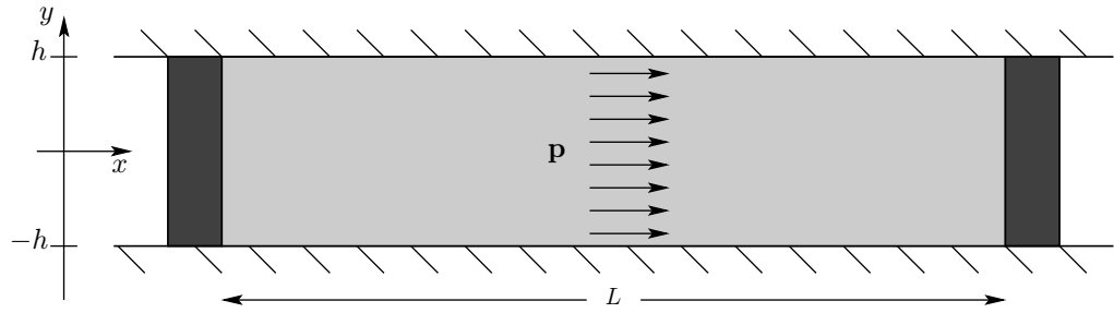
Figure 1. A thin film of active gel positioned between two pistons sets itself into motion.
