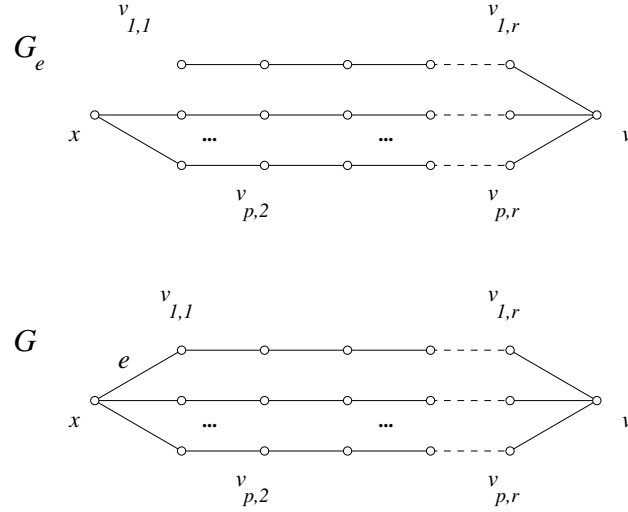
Figure 8: The graphs G_e and G in Proposition 24.
