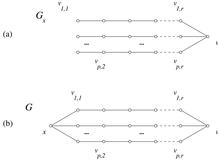
Figure 2: The graphs G_x and G in Proposition 10.
