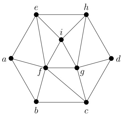
FIGURE 5. A 2-bidismantlable graph G \notin CWW(2)
