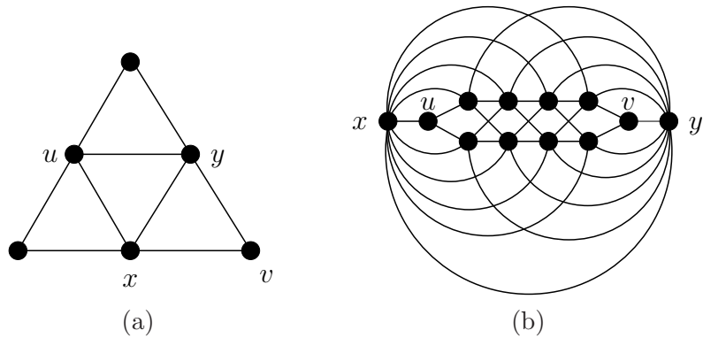
FIGURE 3. Two graphs in (a) CWW(k) \setminus CWR(k) , k \geq 2 and (b) CWW(4) \setminus CWW(5) .
