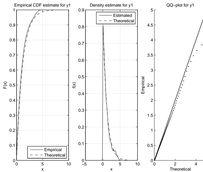
Figure 1: Comparison between the numerically computed distribution with exact distribution. The left figure shows the comparison between the empirical cumulative distribution function (cdf) and the exact cdf. The middle figure makes a comparison between the estimated density function and the exact density function. And the right figure is the qq-plot of the empirical quantiles versus the exact quantiles.
