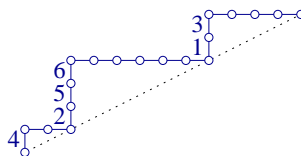
FIGURE 3. A labelled 2-ballot path.
