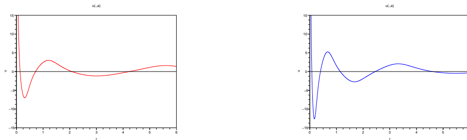
FIGURE 2. Positivity set of u(., a) with two ( a = 50 , left) and three ( a = 90 , right) connected components ( d = 3 ).
