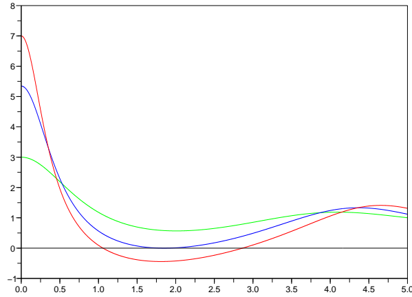
FIGURE 1. Behaviour of u(., a) for a > a_c , a = a_c and a < a_c .
