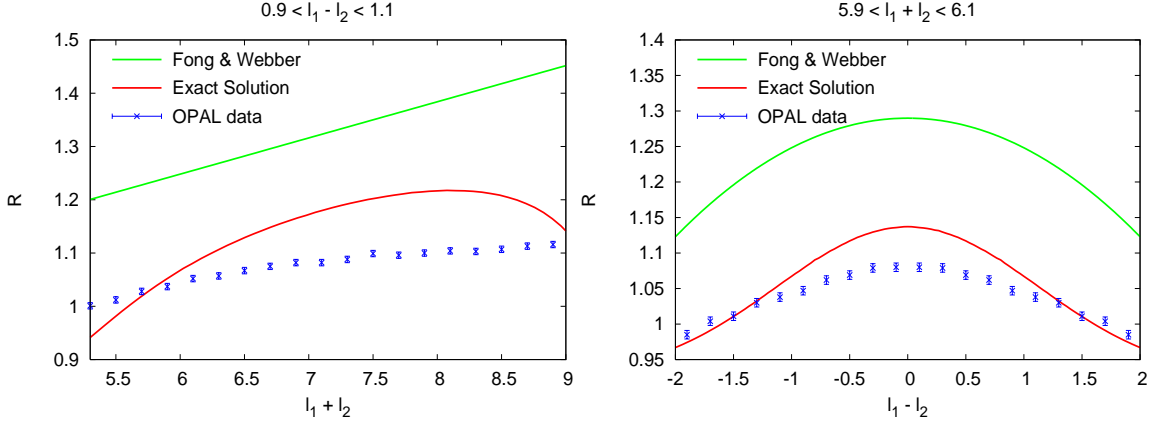
Figure 2: Two-particle correlations in two quark jets \left(R = \frac{1}{2} + \frac{1}{2}C_Q^{(2)}\right) [5] in the process e^+e^- \rightarrow q\bar{q} as a function of \ell_1 + \ell_2 = |\ln(x_1x_2)| for \ell_1 - \ell_2 = \ln(x_2/x_1) = 1.0 (left) and \ell_1 - \ell_2 = |\ln(x_2/x_1)| for \ell_1 + \ell_2 = \ln(x_1x_2) = 6.0 (right).
