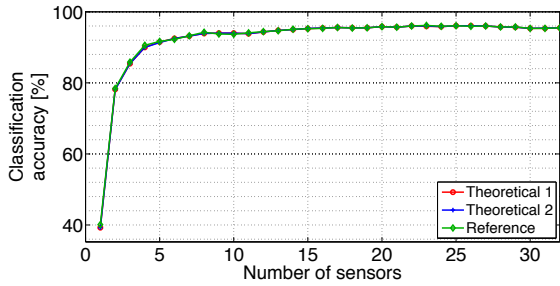
Figure 1: Average classification accuracy after 10 repetitions with respect to the number of selected sensors.
