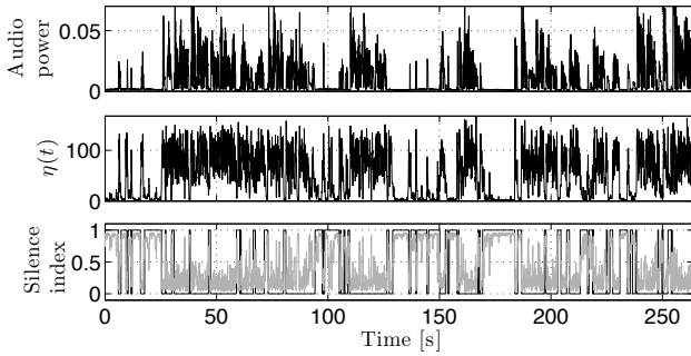
Figure 5: Illustration of visual voice activity detector. In the bottom plot, the black line is the ground truth of silence (1 means silence while 0 means speech) and the grey line is the visual probability of silence p_V(t) (2), with \alpha = 2 and \beta = -1 .
