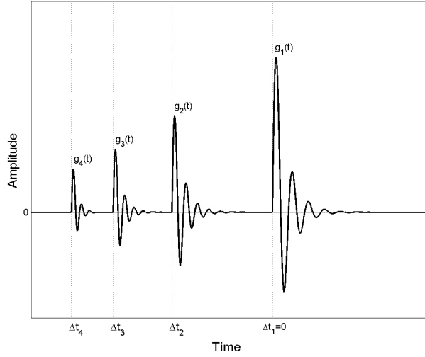
Figure 2: Separation of the different order of non-linearity after convolution with y(t) .
