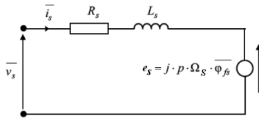
Fig. 4. SM-PM's Behn-Eschenburg equivalent electrical model.
