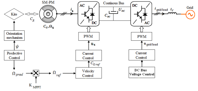
Fig. 7. General control scheme of the KGS.
