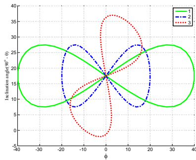
Fig. 7. Test orbits.
