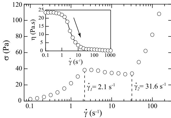
FIG. 9. The flow curve, shear stress \sigma vs shear rate \dot{\gamma} obtained by increasing \dot{\gamma} [ c = 0.1 \text{ mol.L}^{-1} ]. Inset : Viscosity as a function of shear rate. The arrow indicates the shear-thinning behavior [C-VOR 150 Bohlin rheometer, plate-plate geometry, diameter 60 mm, gap 400 \mu\text{m} , waiting time 60 s per point].
