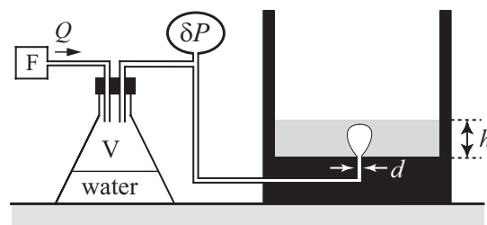
FIG. 1. Experimental setup. A constant air-flow is supplied at the base of a thin layer of micellar fluid by an air-flow controller F (flow-rate Q ), via a chamber of volume V . h is of the order of a typical bubble diameter (a few millimeters to centimeters).
