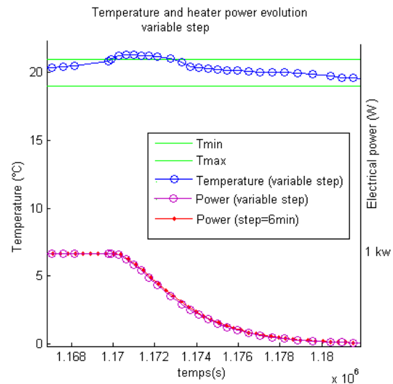
Fig. 6. Variable step time simulation
