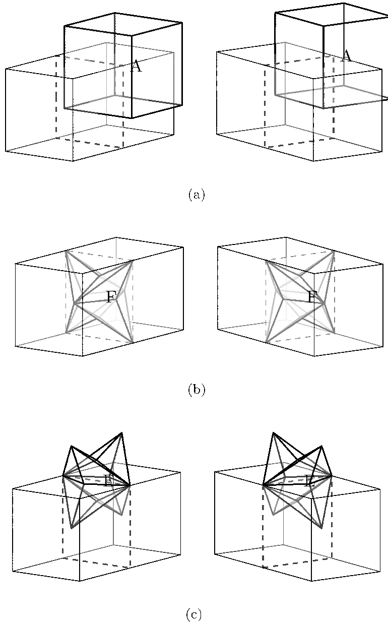
Figure 2: Construction of dual meshes \mathfrak{M}_h^\mathcal{V} and \mathfrak{M}_h^{\mathcal{EF}} from a cubic primal mesh \mathfrak{M}_h^{\mathcal{P}} . In (a), (b) and (c) we show two adjacent cubic cells of \mathfrak{M}_h^{\mathcal{P}} (thin solid lines) and one dual cell (thick solid line). The left and the right plots show the same group of two primary cells and one dual cell from two different viewpoints. The interface separating the two primary cells in all plots is drawn using dashed lines. In plot (a) we show a dual cell of type vertex , i.e., a cell that belongs to \mathfrak{M}_h^\mathcal{V} ; in plot (b) we show a dual cell of type face and in plot (c) we show a dual cell of type edge , i.e., cells that belong to \mathfrak{M}_h^{\mathcal{EF}} .
