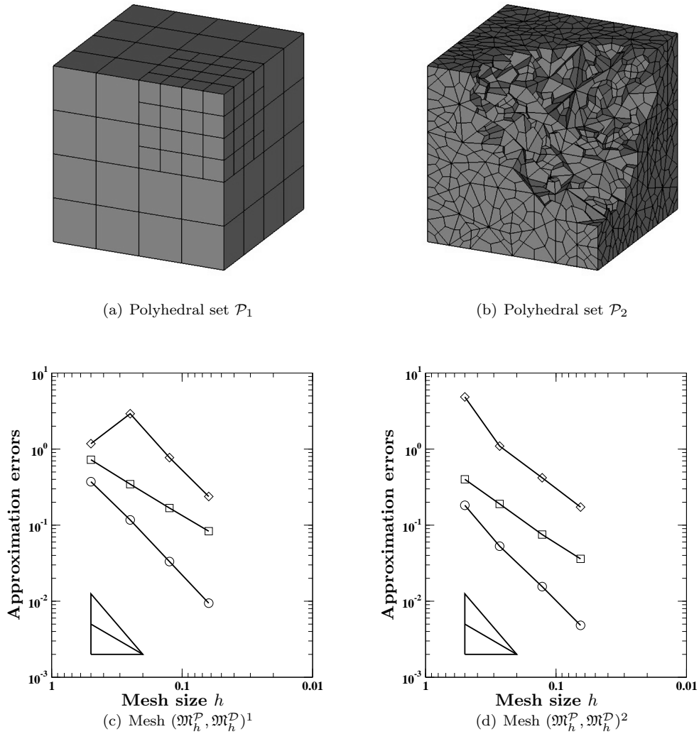
Figure 3: Accuracy test. Plots (a)-(b) display the polyhedral sets \mathcal{P}^1 and \mathcal{P}^2 of the first mesh sets of the two mesh families (\mathfrak{M}_h^{\mathcal{T}}, \mathfrak{M}_h^{\mathcal{D}})_h^1 and (\mathfrak{M}_h^{\mathcal{T}}, \mathfrak{M}_h^{\mathcal{D}})_h^2 used in the accuracy tests. In plot (b), a part of the cells around vertex (1, 1, 1) has been removed to show the interior. The parameters of all the meshes used in the simulation are reported in Table 1. Plots (c) – (d) show the approximation errors for the viscosity field \eta given by (146). In each plot, we report \mathbf{Error}(\mathbf{u}) (circles), see equation (148), \mathbf{Error}(\nabla(\mathbf{u})) (squares), see equation (149), \mathbf{Error}(p) (diamonds), see equation (150), and two straight lines showing the theoretical slopes \mathcal{O}(h) and \mathcal{O}(h^2) .
