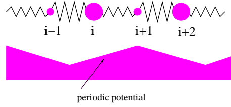
Figure 1: The FK model with n = 2 type of particles (and of springs) and an interaction up to the m = 1 neighbours
