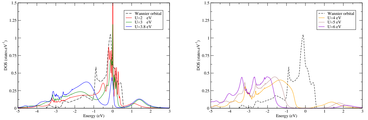
Figure 5.28: LDA+DMFT spectral functions of the d_{xy} Wannier orbital in undistorted \text{Sr}_2\text{IrO}_4 without spin-orbit coupling for U=2, 3, and 3.8 eV (left panel) and U=4, 5 and 6 eV (right panel). The calculations were performed at T=300 K ( \beta = 40 eV ^{-1} ) and with J=0.2 eV. The LDA DOS is shown as dashed line.
