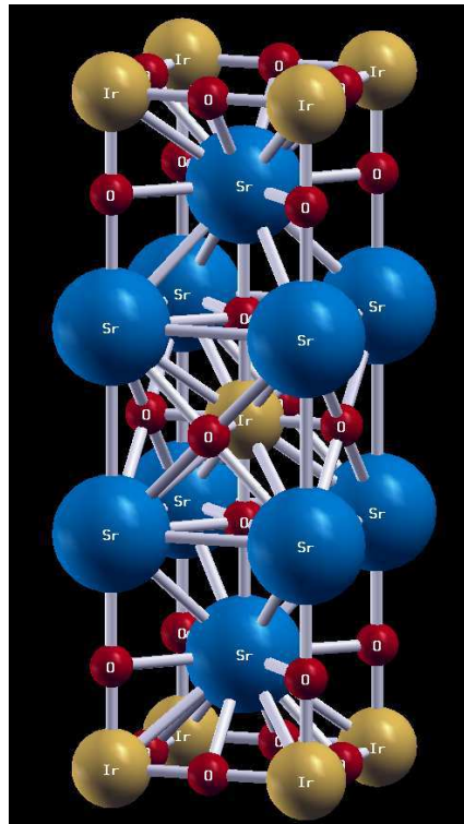
Figure 5.3: Conventional unit cell of Sr 2 IrO 4 in the "undistorted" K 2 NiF 4 -type structure ( I4/mmm symmetry). The blue spheres stand for the strontium ions (Sr), the golden ones for Iridium (Ir) and the red ones for Oxygen (O). The covalent radius of each atomic species was used to set the size of the representing spheres. This picture was obtained with the software Xcrysden.
