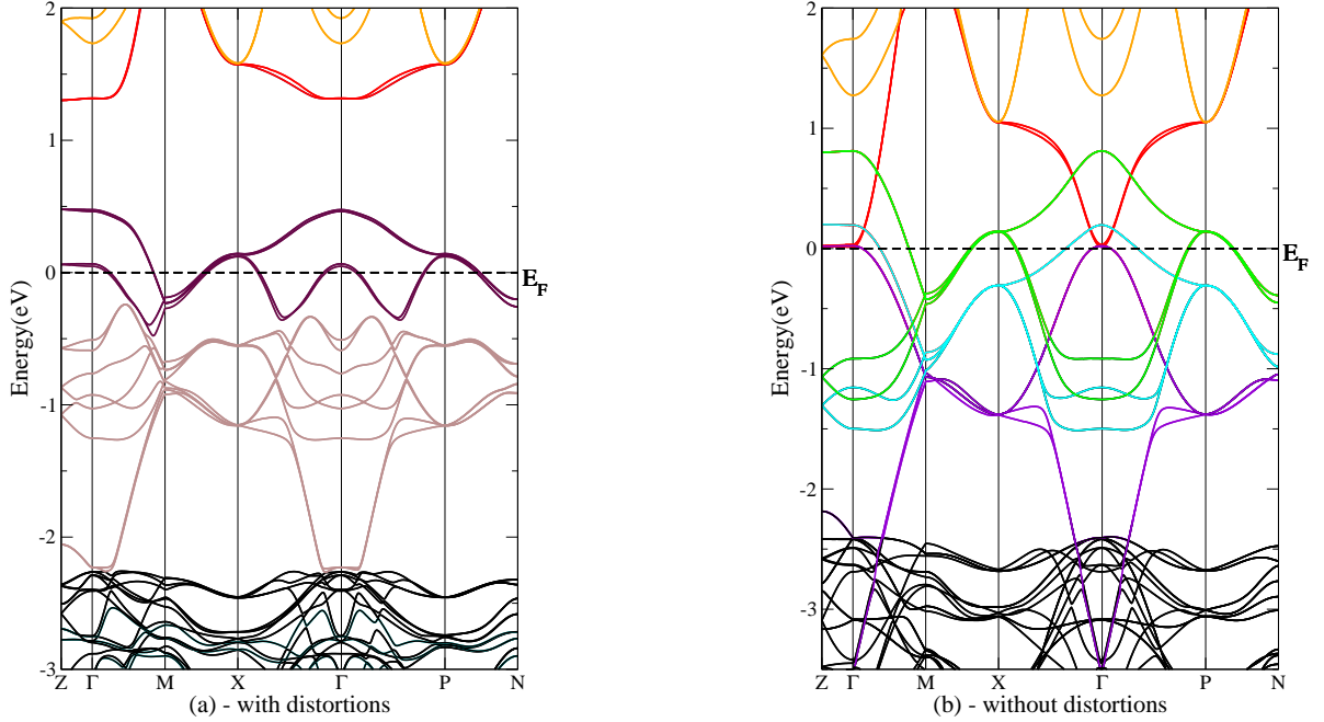
Figure 5.24: Comparison of the Kohn-Sham band structure between distorted Sr 2 IrO 4 (panel a) and undistorted Sr 2 IrO 4 (panel b) with the spin-orbit coupling. Both band structures are represented along the same \mathbf{k} -path (in the distorted I4_1/acd symmetry). The hybridization between the d_{x^2-y^2} and d_{xy} bands (in red and blue respectively) leads to the formation of the energy gap between 0.4 eV and 1.3 eV.
