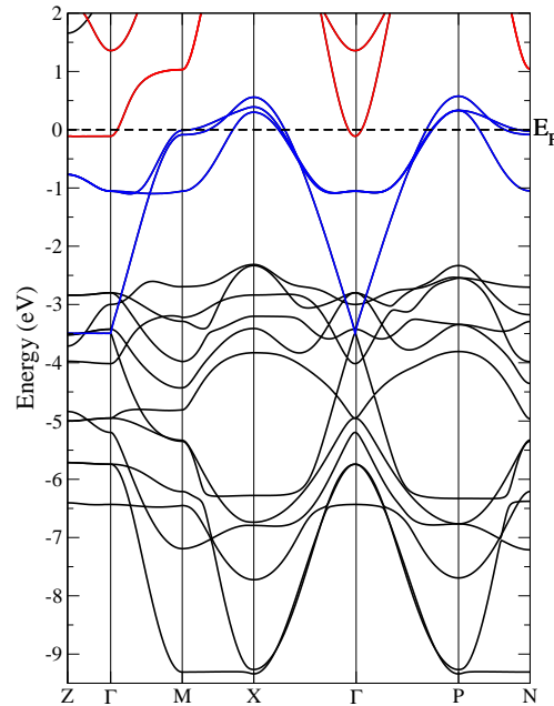
Figure 5.6: Kohn-Sham band structure of \text{Sr}_2\text{IrO}_4 in the undistorted symmetry without spin-orbit coupling. The lower boundary of the energy window is chosen such that the bands up to the Fermi level contain the 29 valence electrons. In blue the t_{2g} bands, in red the e_g and in black the \text{O}2p bands. On \Gamma Z there is almost no dispersion, confirming the two-dimensional nature of the material.
