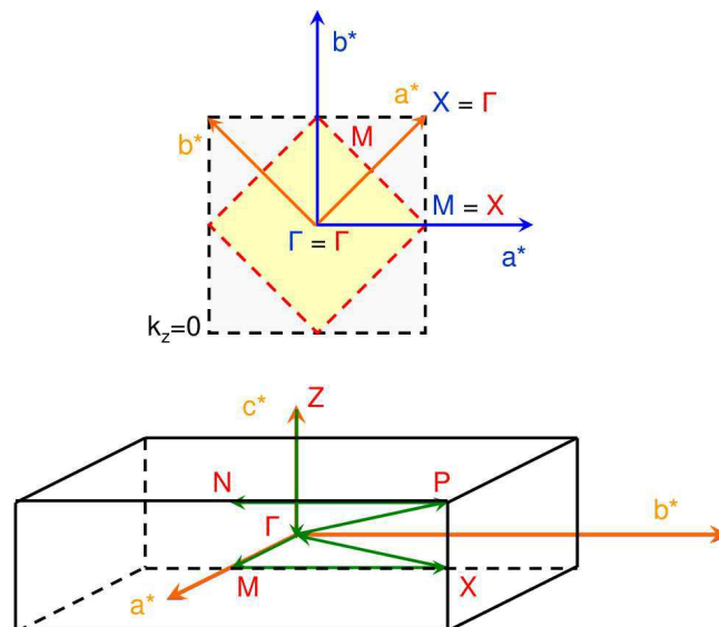
Figure 5.17: Conventional Brillouin zone for \text{Sr}_2\text{IrO}_4 in the distorted symmetry. The high symmetry points are \Gamma(0, 0, 0) , Z(0, 0, 1) , M(0.5, 0, 0) , X(0.5, 0.5, 0) , P(0.5, 0.5, 0.5) and N(0.5, 0, 0.5) . The green arrows depict the \mathbf{k} -path which will be used to represent the electronic band structure in the following. The upper part depicts the correspondence between the distorted Brillouin zone (in red with orange axes) and the undistorted Brillouin zone (in black with blue axes).
