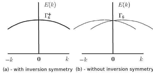
Figure 3.1: Schematic example of the “ Dresselhaus splitting ”. In panel (a), the solid has a center of symmetry and the level is doubly degenerate. In panel (b), the solid has no center of inversion and the Dresselhaus splitting occurs.
