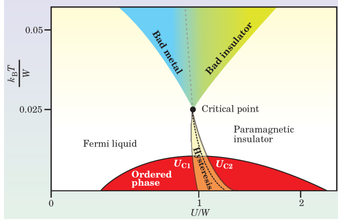
Figure 1.3: Schematic phase diagram of the one band half-filled Hubbard model (1.34) within DMFT. The axes correspond to the temperature T and the Coulomb repulsion U . Energies are normalized by the bandwidth of the model W = 2D . From [99].
