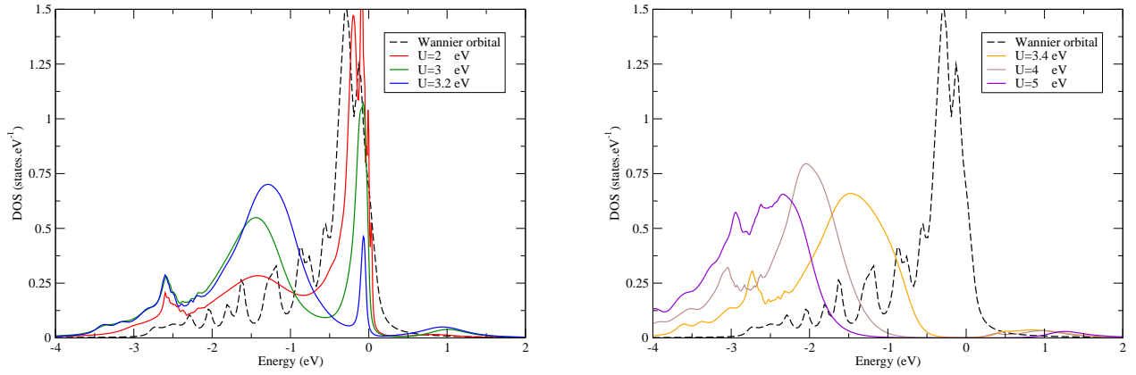
Figure 5.32: LDA+DMFT spectral functions of the d_{xy} Wannier orbital in distorted \text{Sr}_2\text{IrO}_4 without spin-orbit coupling for U=2, 3, and 3.2 eV (left picture) and U=3.4, 4 and 5 eV (right picture).
