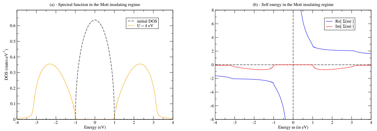
Figure 1.5: Same as figure 1.4, but with U=4 eV.
