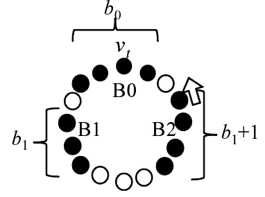
Figure 6: Semi-block leader C_{sbl}(b_0, b_1)
