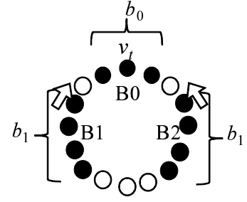
Figure 3: Block leader C_{bl}(b_0, b_1)
