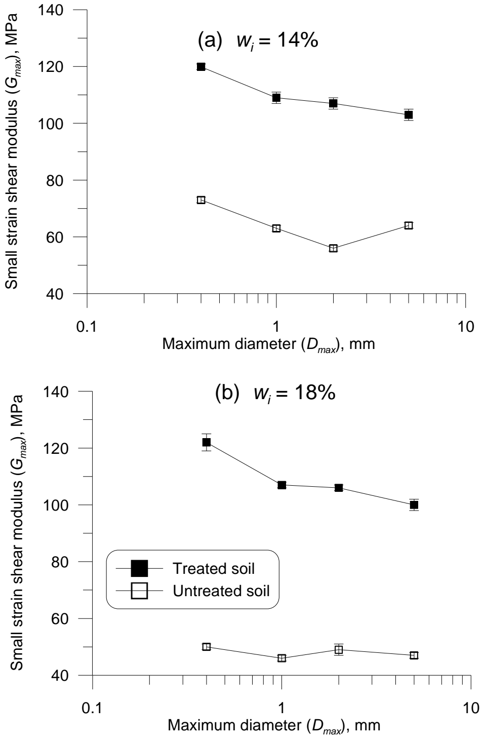
Figure 6. Small strain shear modulus after stabilization versus maximum aggregates diameter
