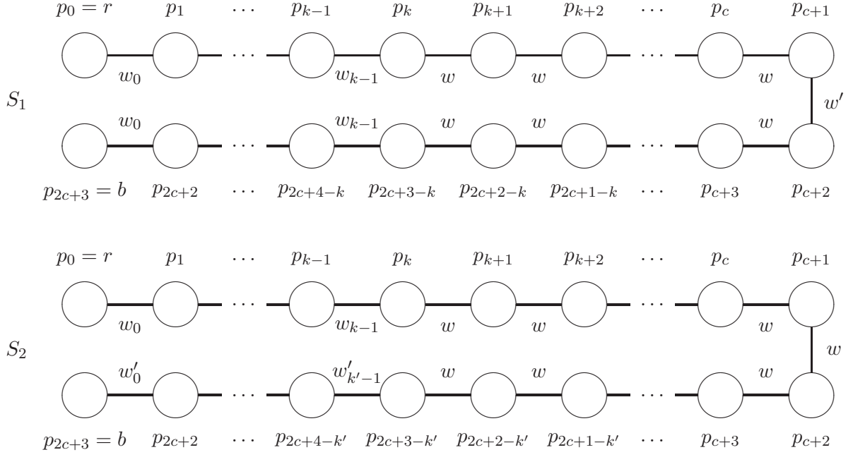
Figure 2: Configurations used in proof of Theorem 8, cases 2 and 3.
