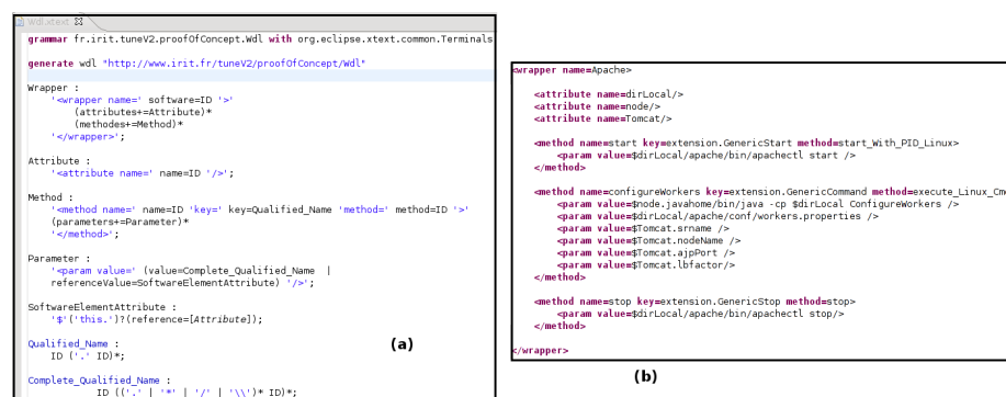
Fig. 5. (a) Wrapping Description Language (b) J2EE WDL
