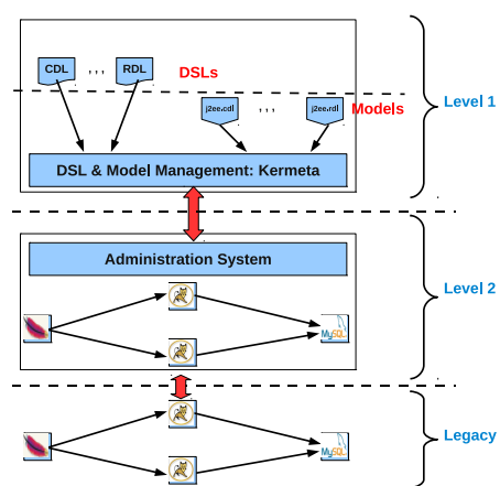
Fig. 9. DSL execution
