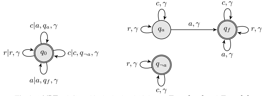
Fig. 1. A VPT_{ia} (left) and its look-ahead (right) on \Sigma_c = \{c, a\} and \Sigma_r = \{r\}
