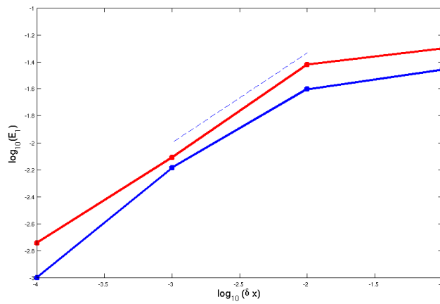
Figure 9: Convergence in space for \mathcal{I}_{\delta x}^1 (red) and \mathcal{I}_{\delta x}^2 (blue). Dotted line has slope 2/3.
