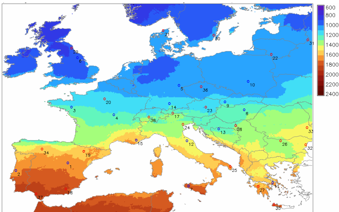
Fig. 1. Yearly sum of global irradiation on horizontal surface – average of 6 databases: Meteonorm v.6, ESRA, PVGIS, NASA SSE v.6, Satel-Light and HelioClim-2 [ \text{kWh/m}^2 ]. Results for 37 randomly selected sites are shown in Fig. 3.
