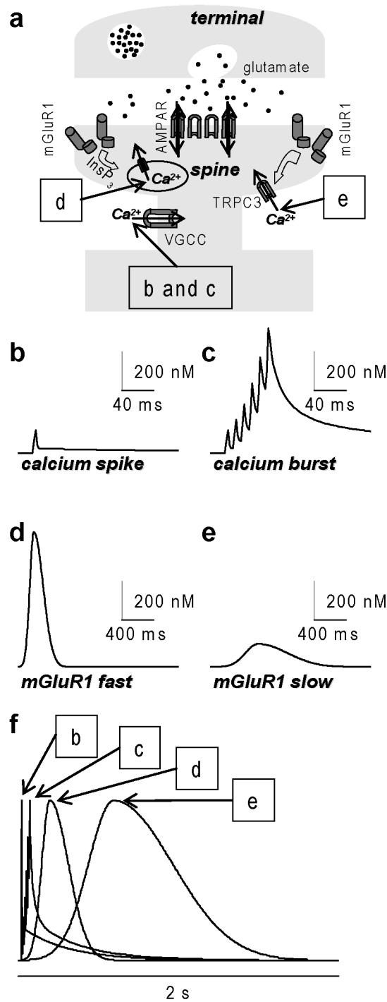
Fig.2. Schematic of four [Ca^{2+}]_i signals associated with excitatory synaptic transmission. (a) Associated with glutamate release from presynaptic terminals and depolarisation due to AMPA receptor (AMPA) activation, [Ca^{2+}]_i can elevate via Ca^{2+} entry through VGCCs (signals b and c), via Ca^{2+} release from stores triggered by mGluR1 activation and InsP_3 (signal d) and via Ca^{2+} entry through TRPC3 triggered by mGluR1 activation (signal e). (b) [Ca^{2+}]_i signal associated with one calcium spike: peak ~100-200 nM, duration ~10 ms; estimate from [14]. (c) [Ca^{2+}]_i signal
