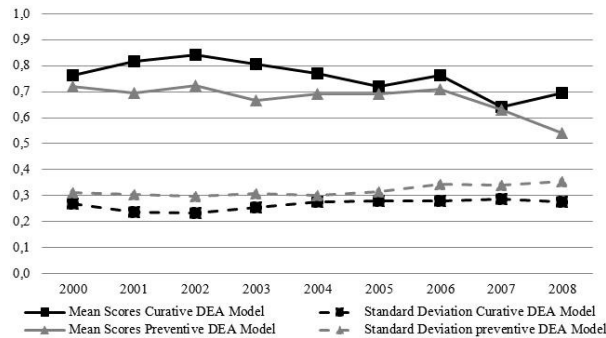
Fig.1 Evolution of THs' technical efficiency scores over the period 2000-2008
