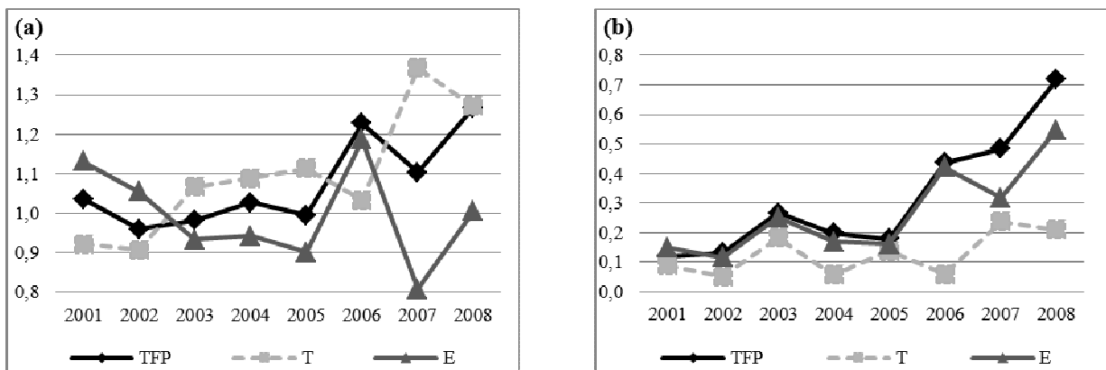
Fig.2 Evolution of mean (a) and of the standard deviation (b) of the Malmquist index and its components for the Curative DEA Model
