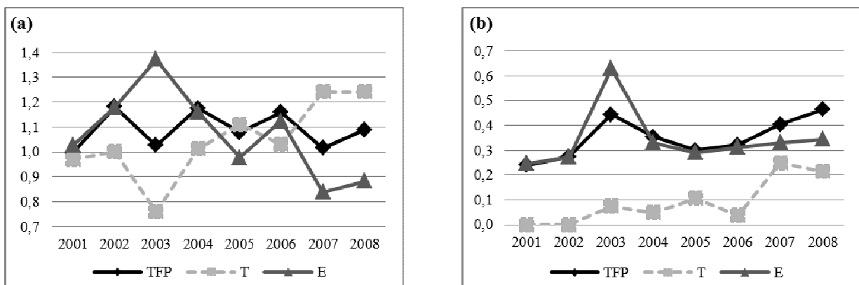
Fig.3 Evolution of mean (a) and of the standard deviation (b) of the Malmquist index and its components for the Preventive DEA Model
