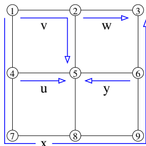
(b) Routing R' .
