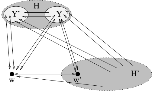
(a) General shape of a (2, w) -digraph
