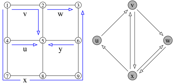
(f) Remove the agent from vertex x and process it, i.e., restore and route request x .
