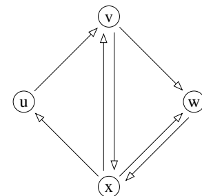
(c) Dependency digraph D .
