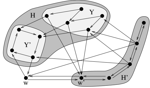
(b) Example of a (2, w) -digraph
