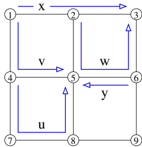
(a) Routing R .
