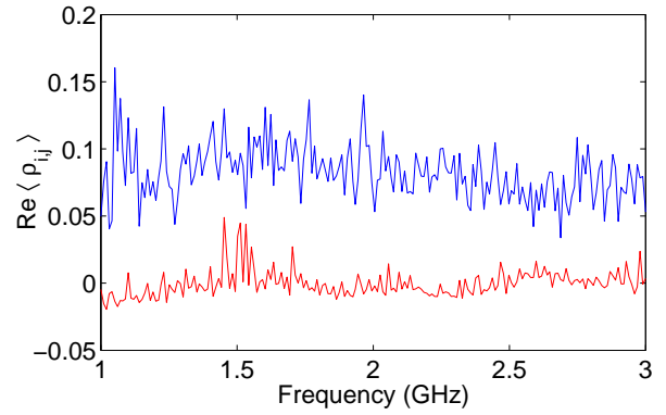
Fig. 1. Residual correlation \bar{\rho} as defined in (9), computed from experimental data when considering the stirrer (blue) or the positions (red) as random realizations of multivariate samples.
