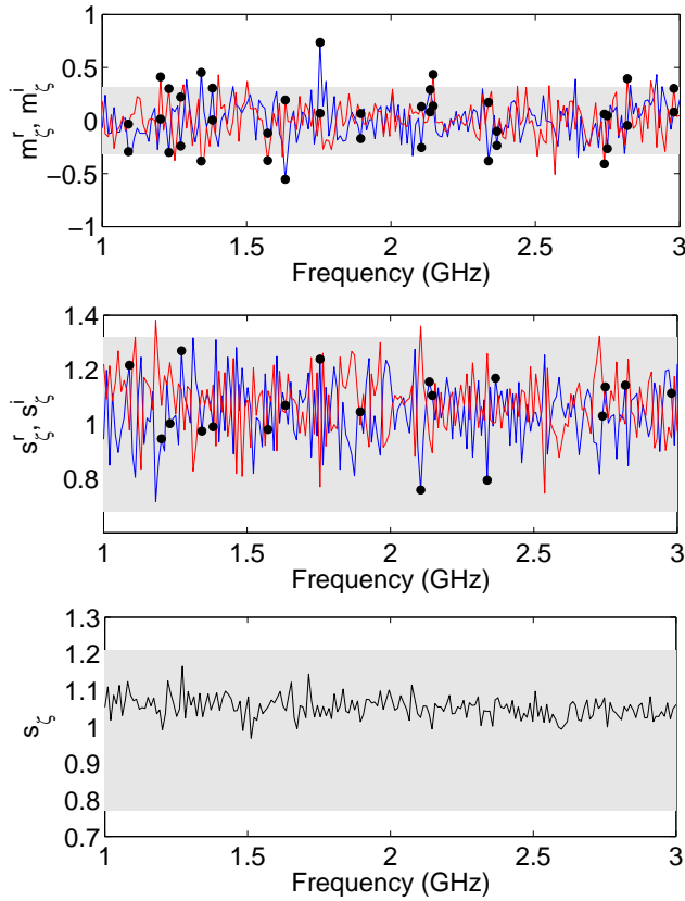
Fig. 2. Empirical moments of \zeta estimated from the N_s multivariate samples: (a) real (blue lines) and imaginary (red lines) parts of the sample average ( m_{\zeta}^r , m_{\zeta}^i ); (b) standard deviations for the real and imaginary parts of \zeta ( s_{\zeta}^r , s_{\zeta}^i ); (c) standard deviation of \zeta ( s_{\zeta} ). Shaded areas represent the expected confidence margin at 95 % probability for the null hypothesis, for a sample population of N_p realizations.
