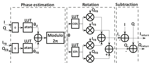
Figure 3. LUT based solution
