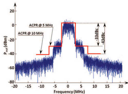
Figure 6. Output spectrum without CFB
