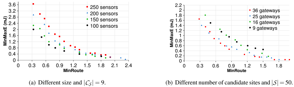
FIGURE 1: Pareto fronts obtained for the random networks tested.
