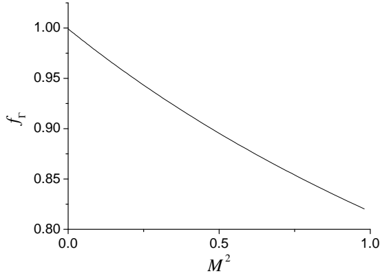
Figure 9. Computed decay rate factor f_\Gamma in Eq. 20 characterising the deviation of ME-induced decay of M from the small M regime of Eq. 19. The empirical fit f_\Gamma=0.999-0.2340M^2+0.0539M^4 is accurate to better than 4\times 10^{-4} .
