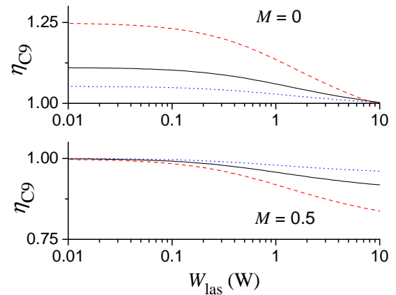
Figure 8. Computed power dependence of the PE of the C_9 line at M=0 (upper graph) and M=0.5 (lower graph) for the same three collisional regimes as in Fig. 7. \eta_{C9} is here the spatial average of the PE in the cell, computed for the same pump beam parameters as in Fig. 5.
