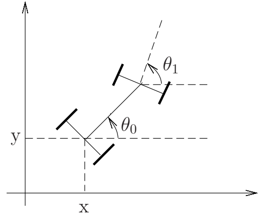
Fig. 2. nonholonomic car
