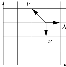
FIGURE 2. A tandem queue.
