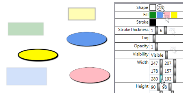
figure 5. The user drags the “width: 280” shared value and drops it on the “shape: circle” shared value. All circles in the selection now have a width set to 280.
