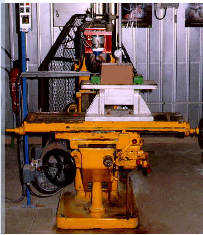
Figure 7 : atmospheric single cutter test stand
