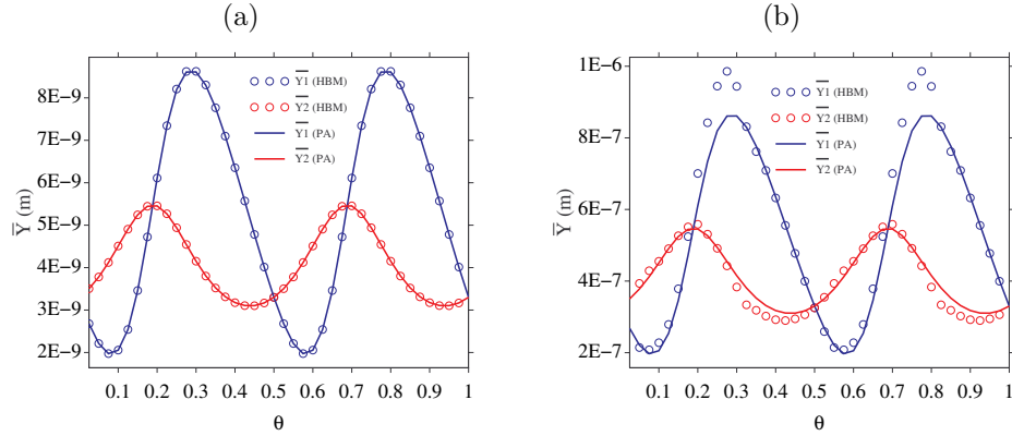
Fig. 8. Evolution of \overline{Y}_k in terms of the ratio \theta = \tau/T . (a): v_0 = 10^{-4} \text{ m/s} ; (b): v_0 = 10^{-3} \text{ m/s} . Circle: harmonic balance method (HBM). Solid line: perturbation analysis (PA), Eq. (4.17).
