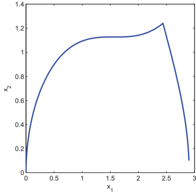
Figure 3.12: Optimal trajectory
