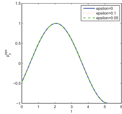
Figure 2.21: p_y^\varepsilon
