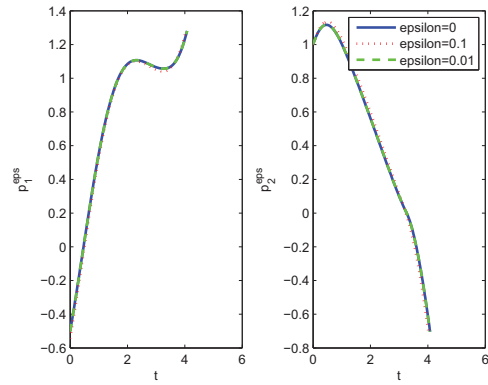
Figure 3.17: Adjoint vector
