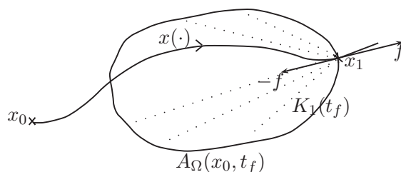
Figure 1.21: Cone K_1(t_f)
