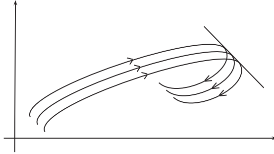
Figure 3.2: Field of extremals in the smooth case
