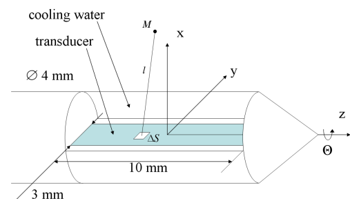
Fig. 1. Ultrasound device geometry and coordinates system.
