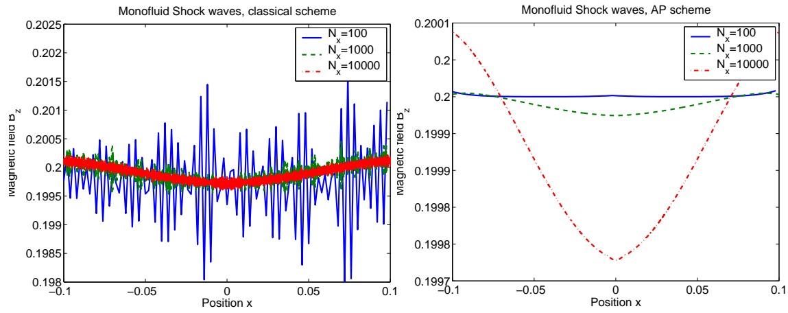
Figure 15: One-fluid shock wave test case with non-zero initial magnetic field. B_z as a function of x at time t = 5 \times 10^{-4} with \lambda = 10^{-4} for the classical scheme (left panel) and AP-scheme (right panel). \Delta x/\lambda respectively equals 0.2, 2 and 20 for N_x = 10000 , N_x = 1000 and N_x = 100 discretization cells.
