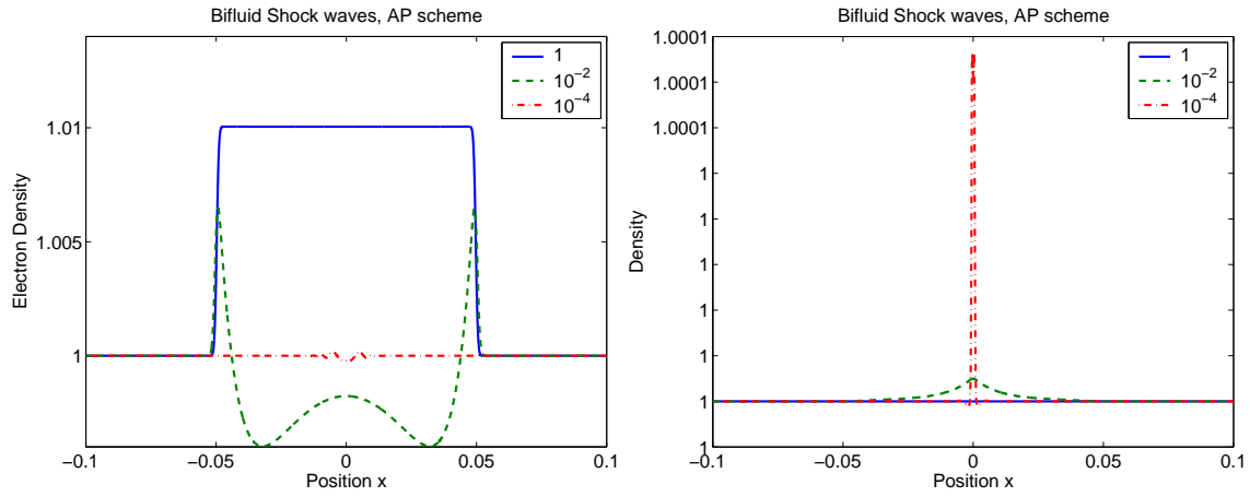
Figure 10: Two-fluid shock wave test case with zero initial magnetic field. n_e (left panel) and n_i (right panel) as functions of x at time t = 5 \times 10^{-4} for \lambda = 1 , \lambda = 10^{-2} and \lambda = 10^{-4} computed with the AP-scheme on N_x = 10^4 space cells.
