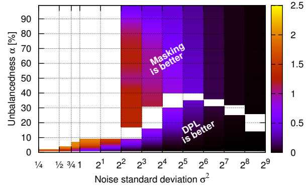
Fig. 3. Plot of domains where either masking or DPL leaks less (units: bit).
