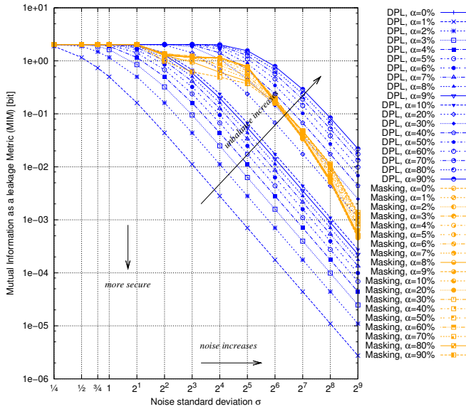
Fig. 2. Comparison between the leakage of DPL and masking countermeasures as a function of the experimental noise, for various \alpha and n = 4 bit.
