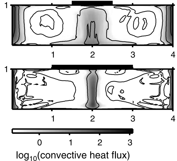
Figure 7. Contour lines of the time-averaged convective heat flux (equation (3)) for Ra = 10^7 with a model of aspect ratio 4. The continental lid has a Biot number B = 10 , and a width (top) 1 or (bottom) 2.
