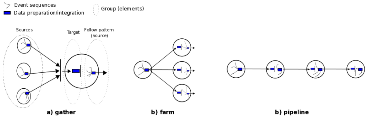
Fig. 2. Invasive Patterns
