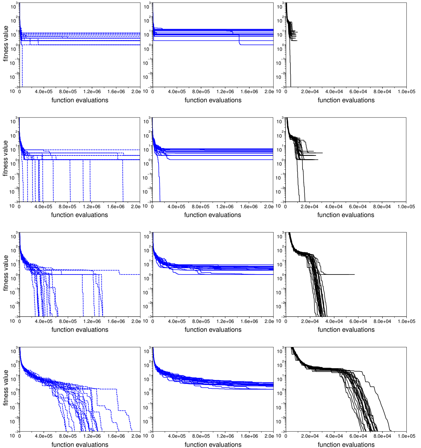
Figure 9: Rastrigin function in 10-D: time evolution of the objective function value of all 21 runs. Left column: s-PSO on the non-rotated Rastrigin function until up to 2 \times 10^6 function evaluations. Middle column: s-PSO on the rotated Rastrigin function until up to 2 \times 10^6 function evaluations. Right column: CMA-ES on the rotated Rastrigin function until up to 10^5 function evaluations. Swarm/population size of 30, 100, 300, 1000 from top to bottom. The CMA-ES was terminated before the maximum number of function evaluations was reached also in the unsuccessful trials.
