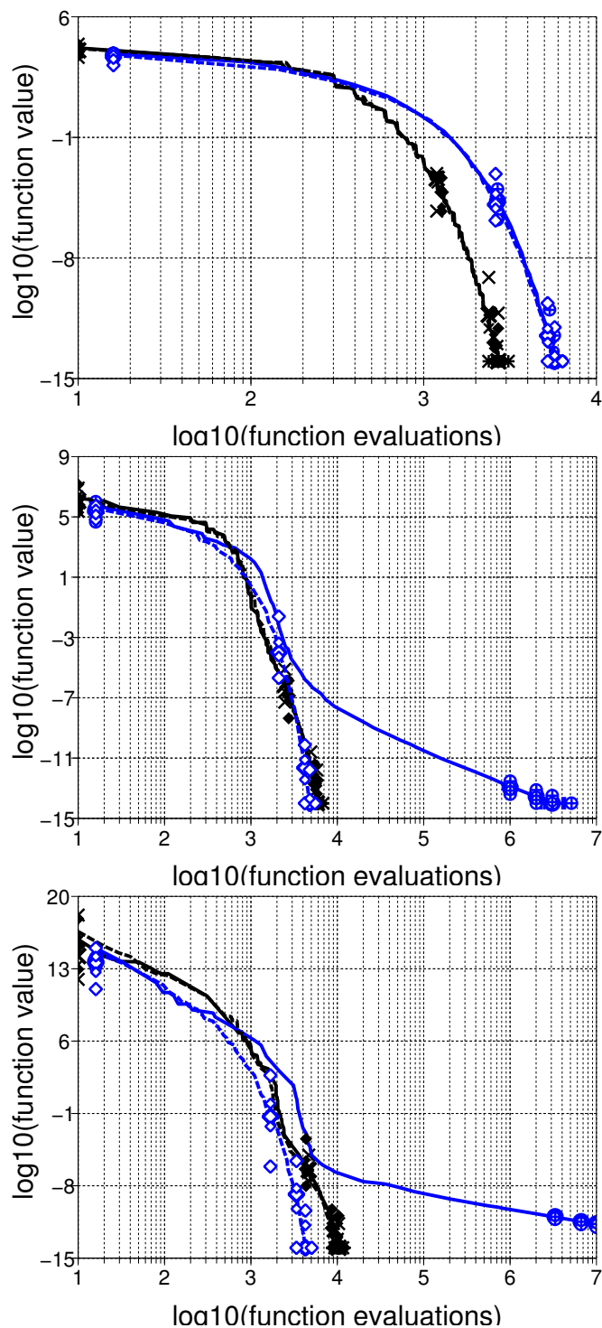
Figure 7: Diff-Powers function in 10-D: time evolution of the median function value, rotated and non-rotated case, with parameter \alpha equals to zero (top), two (middle) and ten (bottom). Small symbols indicate the 25%- and 75%-ile, large symbols indicate smallest and largest value from 21 trials. s-PSO: \oplus, \circ ; CMA-ES: \times, \diamond
