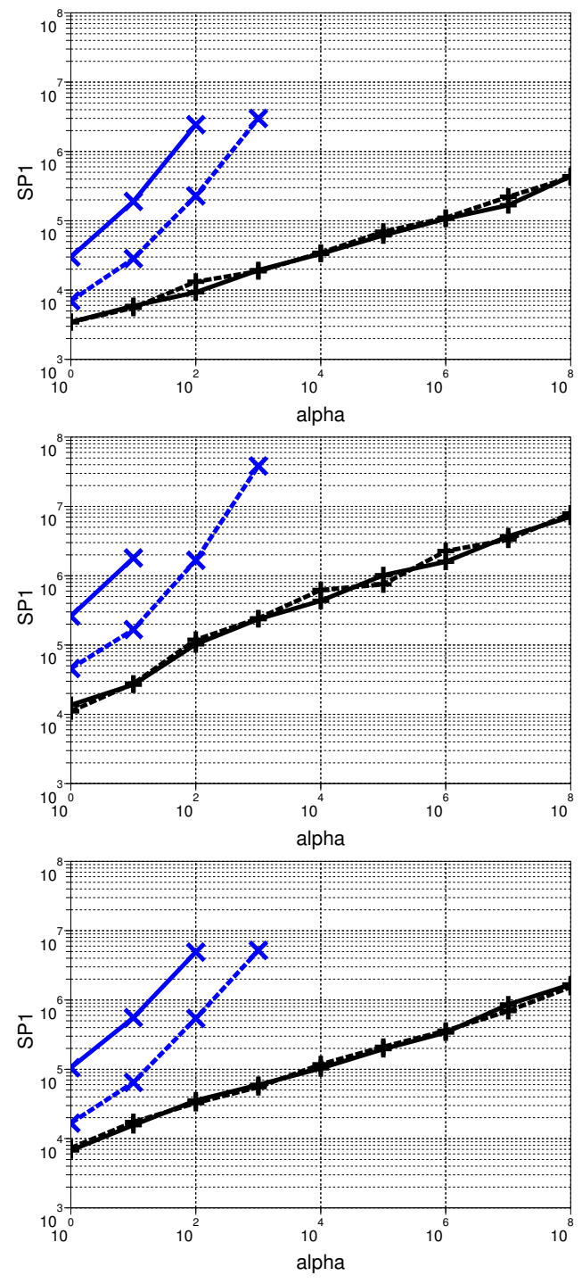
Figure 6: Rosenbrock function: \widehat{SP1} (number of function evaluations) versus conditioning parameter \alpha in 10 (top), 20 (middle), and 40-D (bottom). s-PSO corresponds to the two upper lines in each case. Solid lines: rotated, dashed lines: non-rotated.
