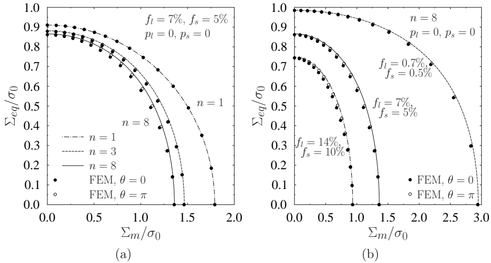
Figure 6: Influence of the nonlinearity exponent n (a) and the void volume fractions f_s and f_l (b) on the macroscopic equipotential surfaces. Comparison between the model predictions and the finite element calculation results. Non pressurized voids ( p_l = p_s = 0 ). (a) n = 1, 3 and 8 , f_l = 7\% , f_s = 5\% . (b) n = 8 , f_l = 0.7\% , 7\% and 14\% with f_s = 0.5\% , 5\% and 10\% , respectively. Results based on the finite element calculations are marked with black filled circles (Lode angle \theta = 0 ) and white circles (Lode angle \theta = \pi ), whereas the results based on the N -layer model are given by lines. N = 20 when f_l = 0.7\% , N = 10 when f_l = 7\% , 14\% .
